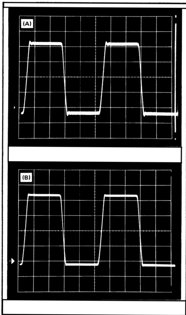
Fig. 2-3. Waveform distortion produced with incorrect probe ground. (A) Eighteen-inch ground strap between generator and oscilloscope. (B) Five-inch ground strap.
