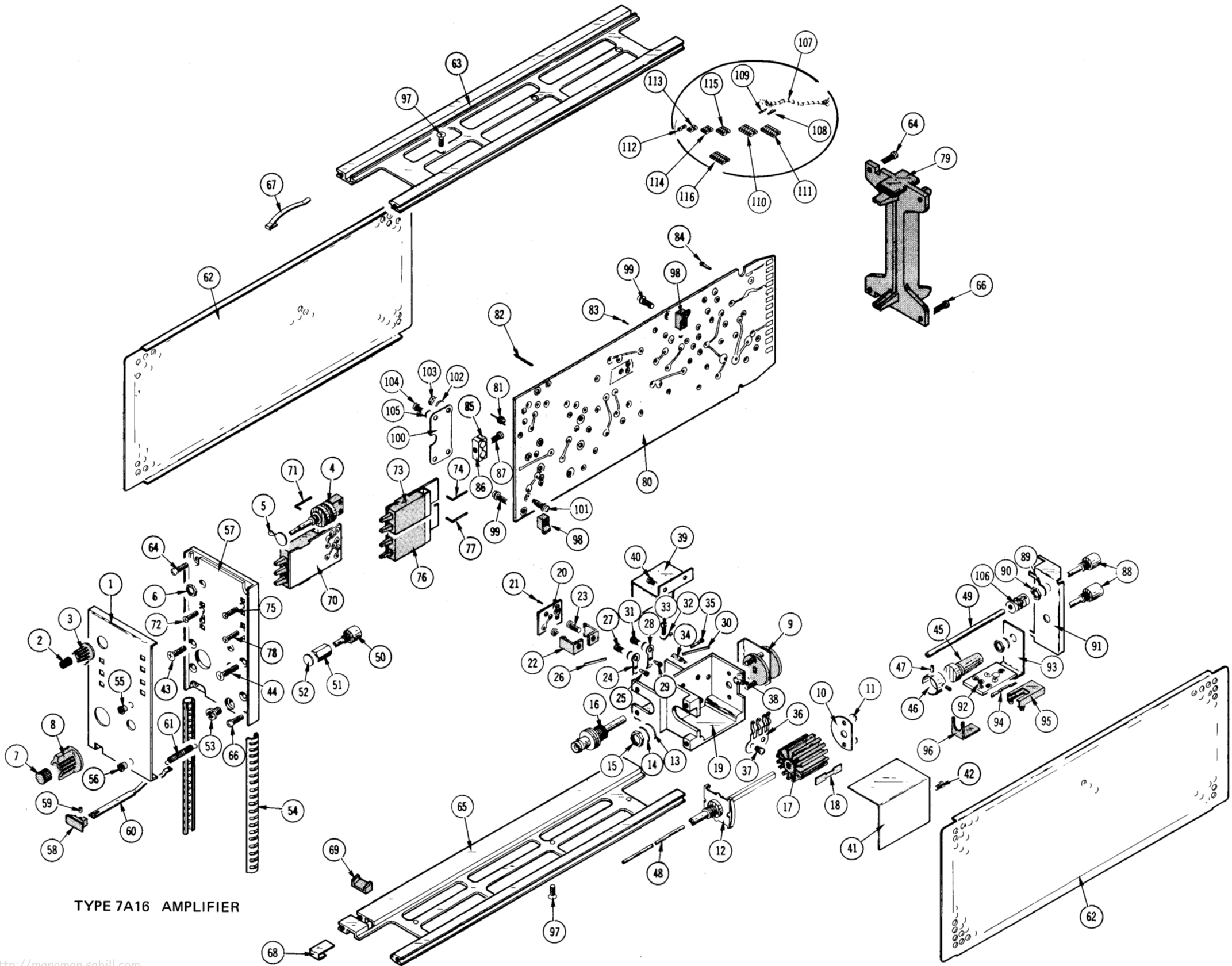
FIGURE 1 EXPLODED
